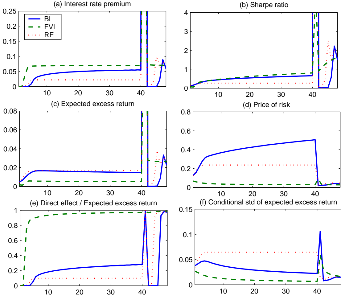
Figure 9: Asset Price Dynamics
