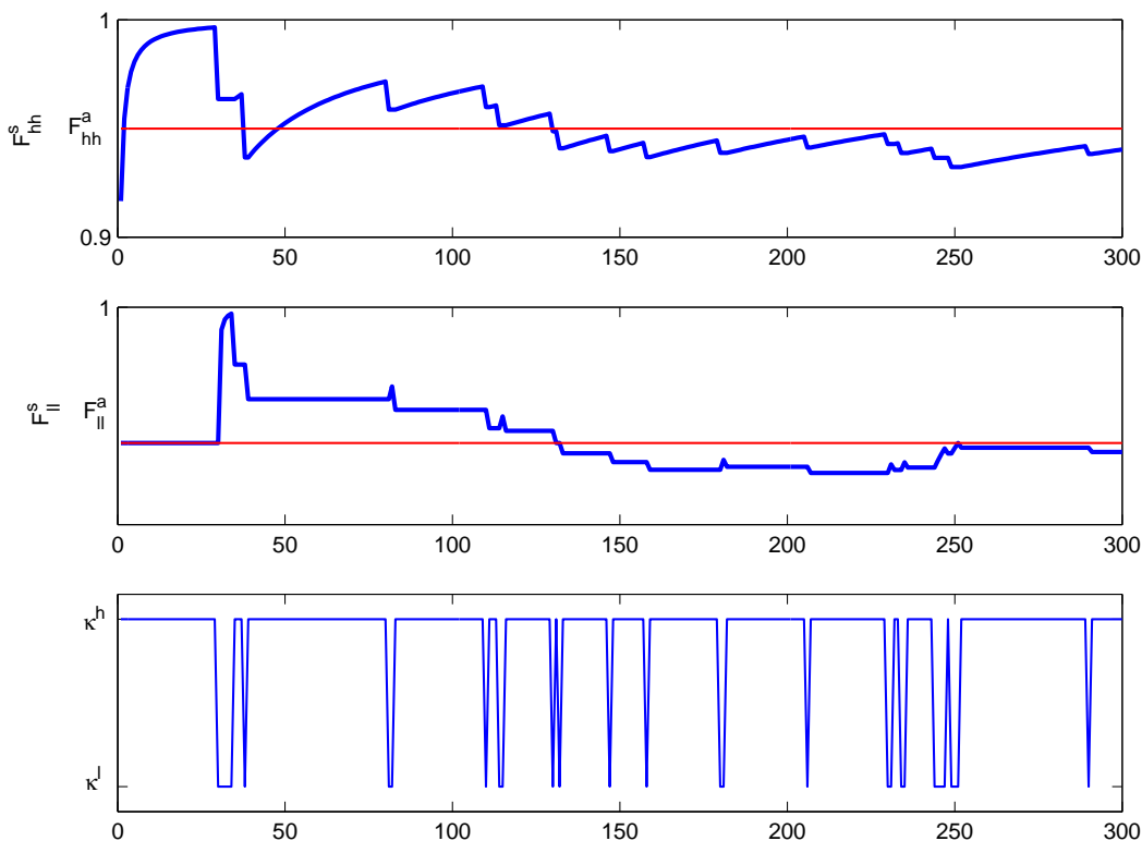
Figure 4: Evolution of Beliefs
