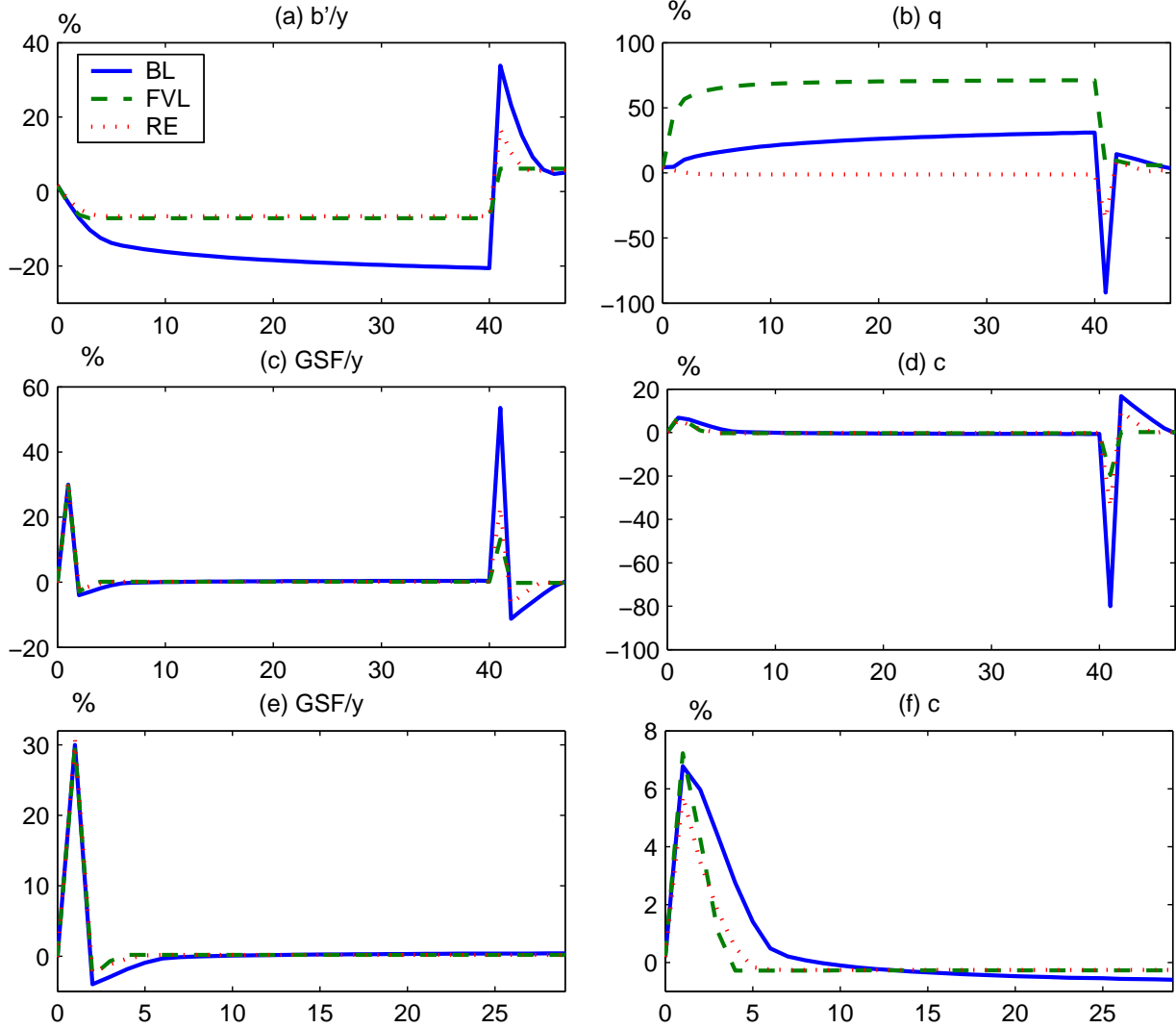
Figure 8: Forecast Functions
