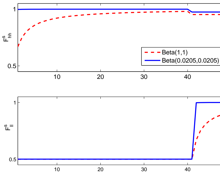
Figure 6: Evolution of Beliefs under Alternative Priors
