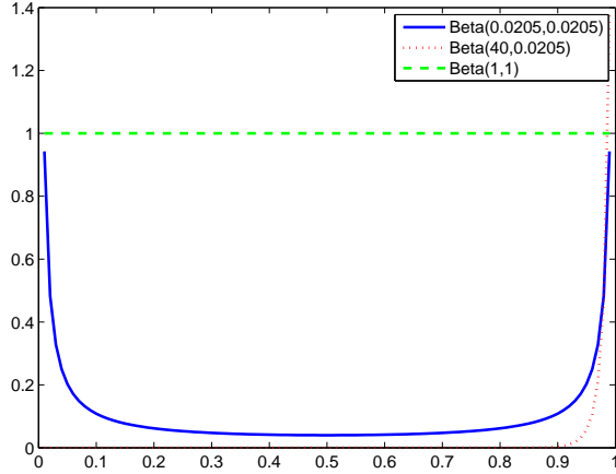
Figure 5: Beta Distributions
