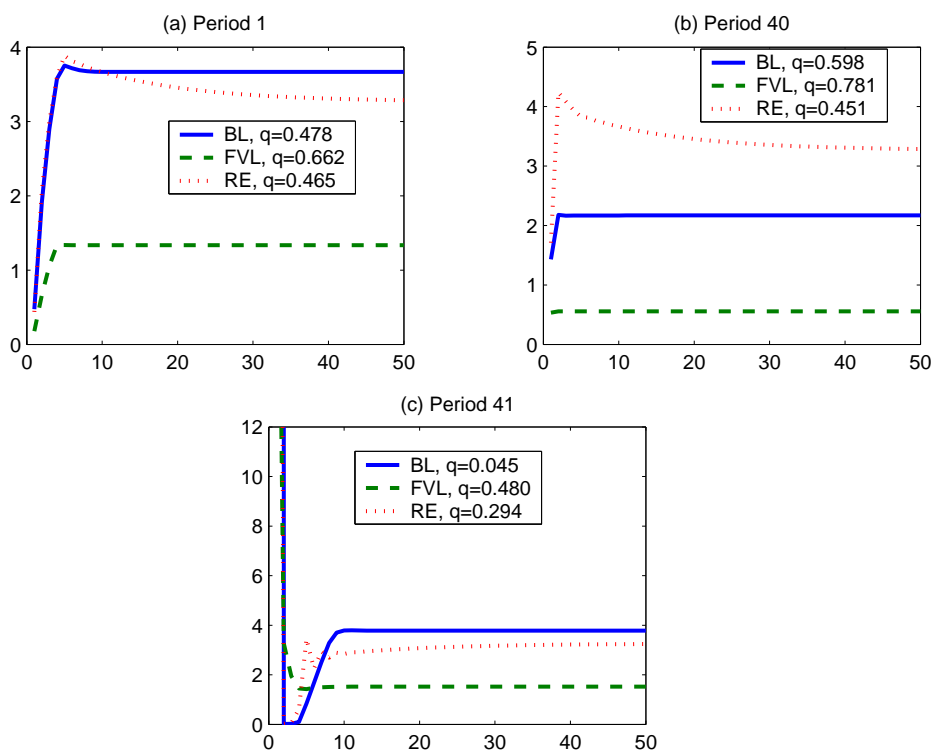
Figure 10: Excess Returns
