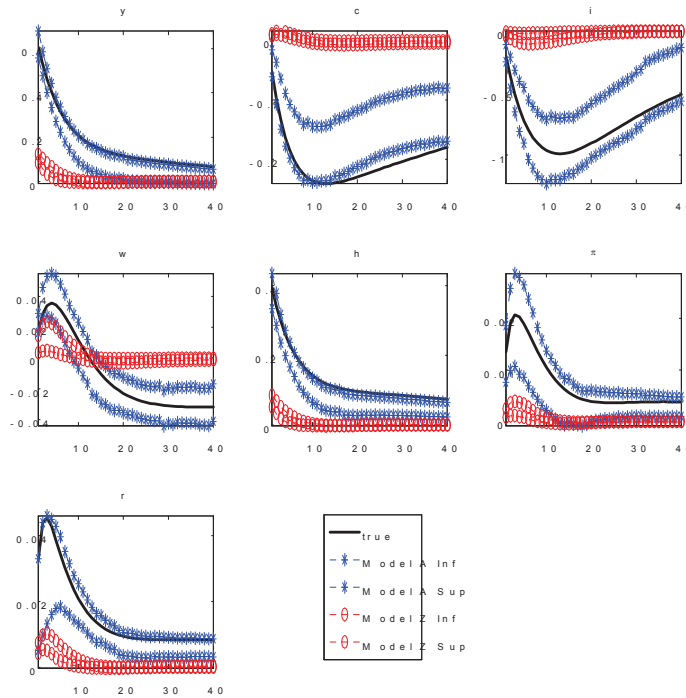
Figure 3: Impulse response to a government spending shock. Stars represent highest 90 percent credible sets for Model A; red circles the highest 90 percent credible sets for Model Z ; the black solid line the true impulse response. From top left to bottom right, are the response of output y , consumption c , investment i , real wage w , hours h , inflation \pi and nominal interest rate r .
