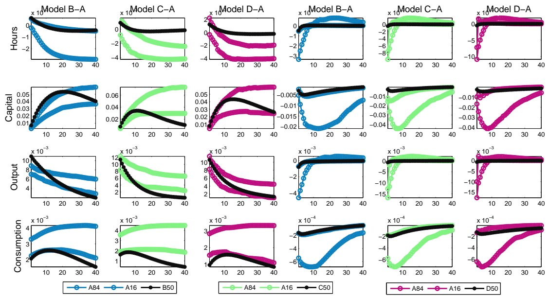
Figure 9: Impulse responses, DGP2 (parameter variations explain 20 percent of output variance)
