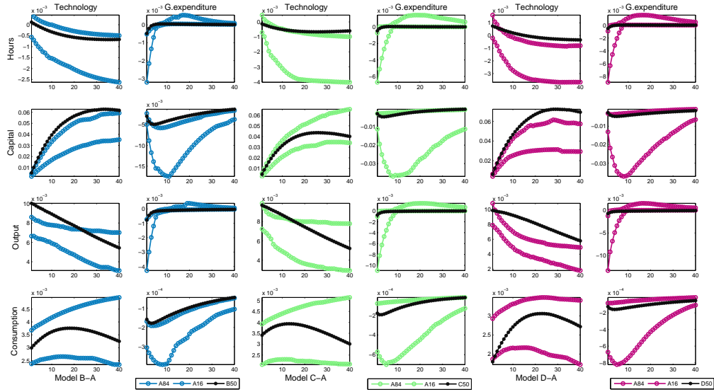
Figure 4: Impulse responses, DGP1
