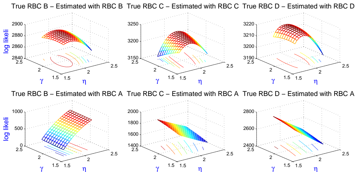
Figure 2: Likelihood surfaces
