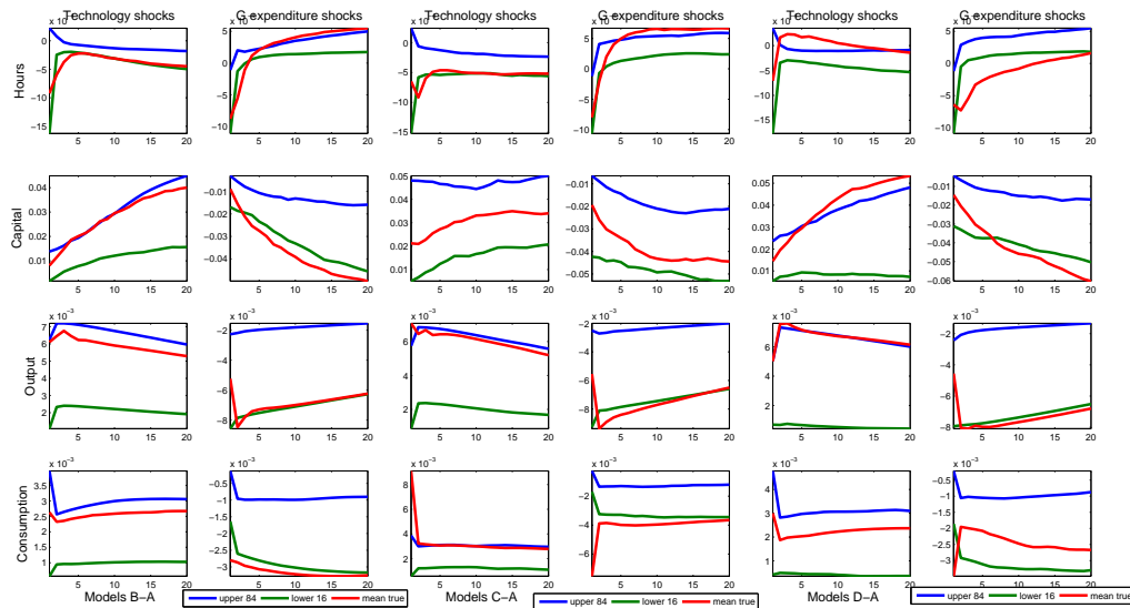
Figure 5: Impulse responses, DGP1, SVAR models.
