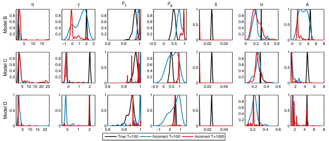
Figure 8: Density of estimates, DGP2 (parameter variations explain 20 percent of output variance).
