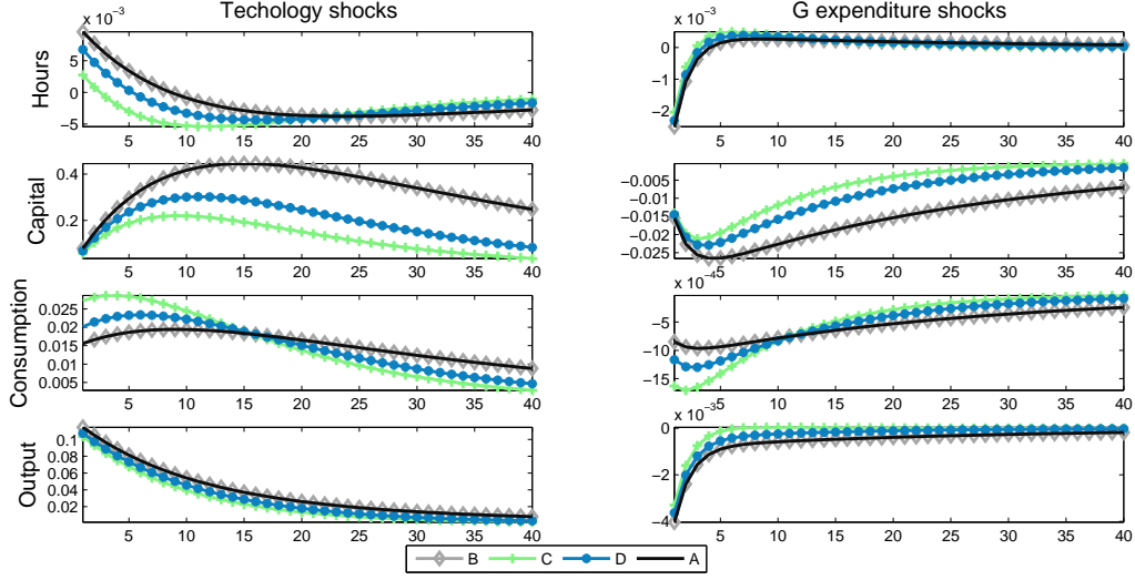
Figure 1: Impulse responses, first order approximation
