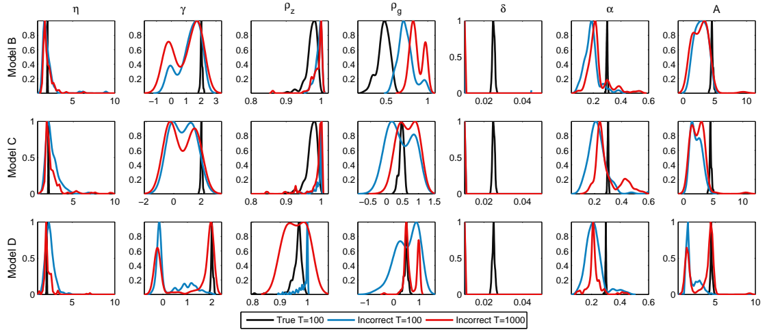
Figure 7: Density of estimates; DGP1 (parameter variations explain 2-5 percent of output variance).
