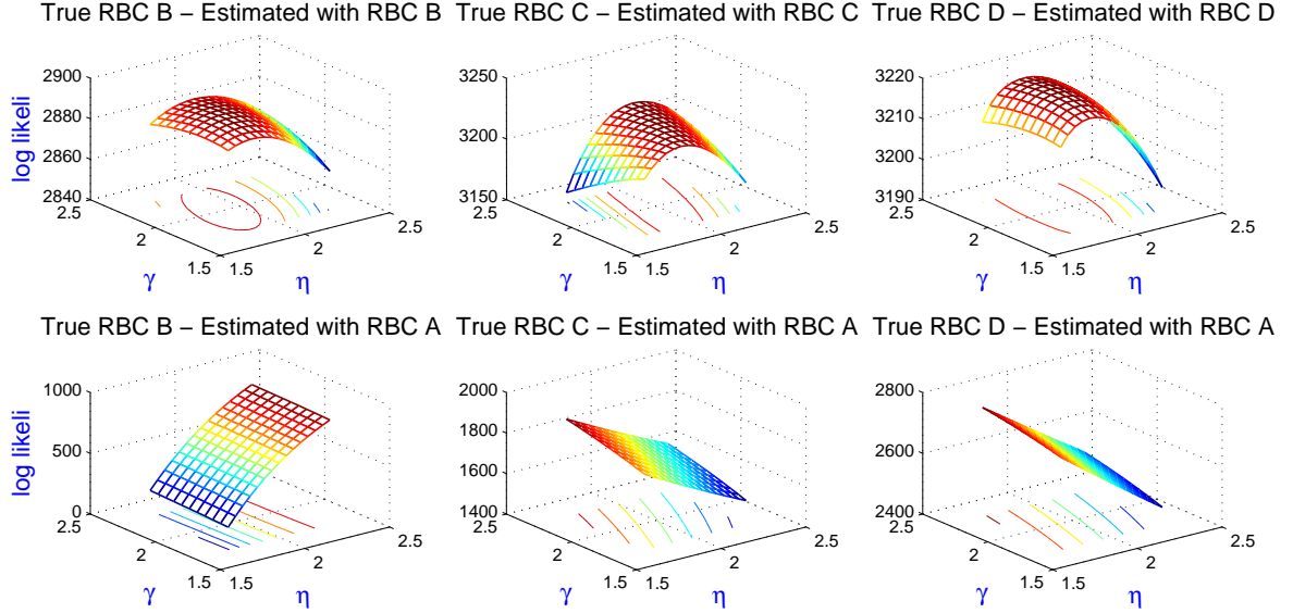
Figure 3: Likelihood surfaces
