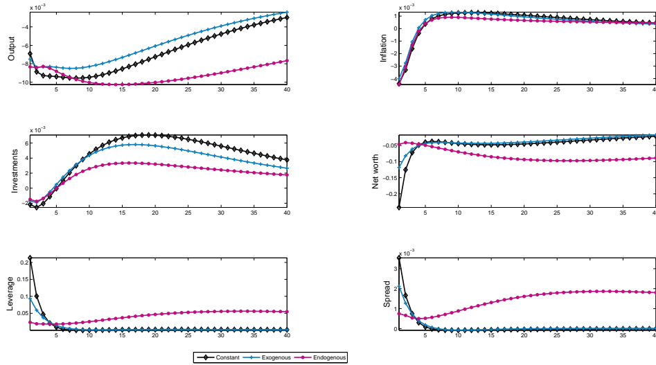
Figure 6: Dynamics in response to a capital quality shock.
