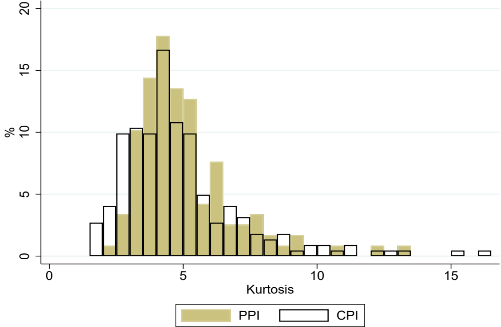
(b) Kurtosis
